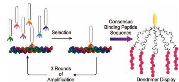
Figure 1. From phage display to dendrimer display: phage display to collagen reveals a consensus binding sequence that is translated into a high affinity, versatile synthetic collagen-specific probe by mimicking the original pentavalent phage architecture on a dendritic wedge.
